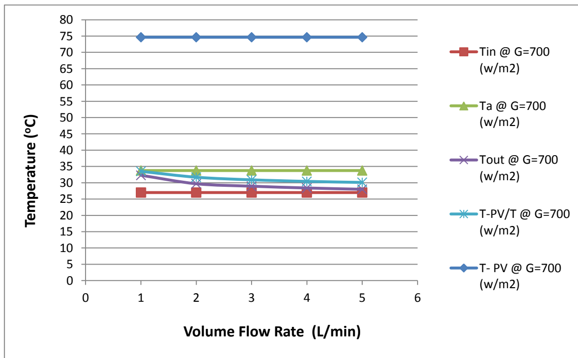
Figure 2. (Ambient, Inlet, Outlet, and PV) Temperatures for Water Based PV/T System Compared with PV Module Temperature for Solar Irradiance of 700 \text{ W}/m^2
